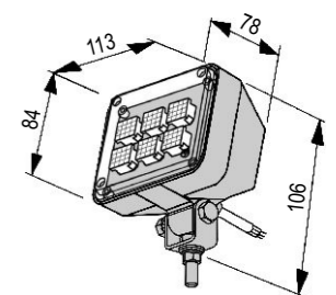
LD116 Advance dimensions (mm) Swivel mounting kit.
