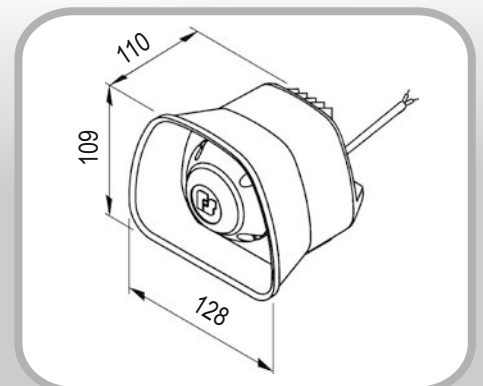
ALS1000-D Speaker dimensions in mm.
