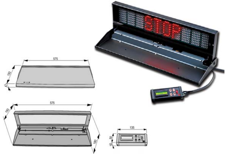
Dimensions Smartsign in mm
